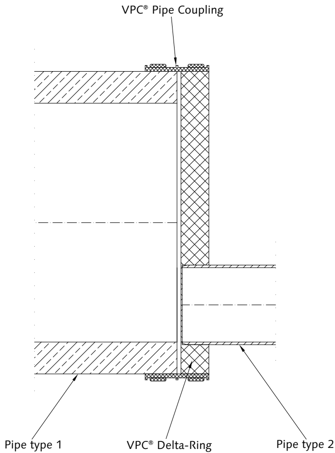
VPC® pipe coupling with VPC® Delta Ring
